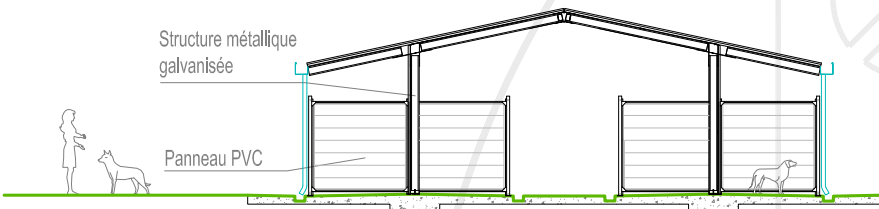
SECTION TRANSVERSALE C-C
